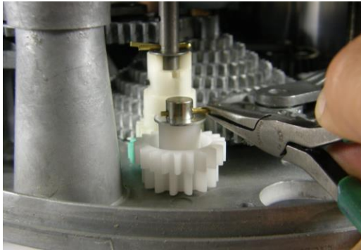
A. Locate the white plastic compound gear and remove and save the cotter pin.
