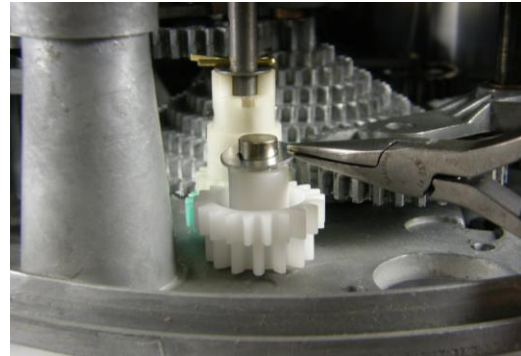
B. Remove and save the top washer which has an outer diameter of 5/8".
