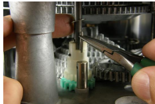
F. Slide the washer up the dollar drive shaft and insert the dollar drive shaft vertical pin (you will need to rotate the gear to get the pin to seat into the bottom gear).
