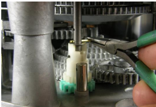
E. Remove the cotter pin from the dollar drive shaft.
