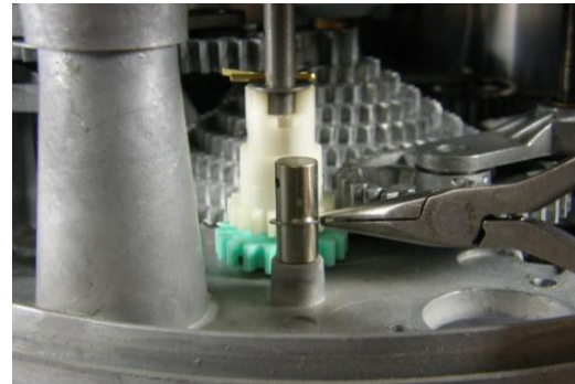
D. Remove and save the bottom washer which has an outer diameter of 5/16".
