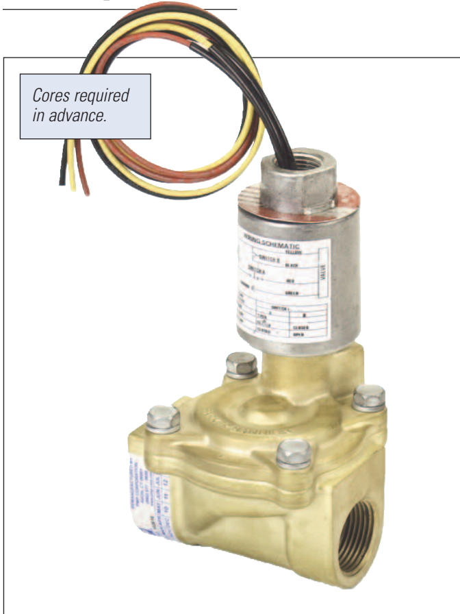
PMP #22057 2-Stage, 1" Threaded with Coil, 3-Wire MFG #067034
