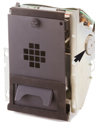
Gilbarco CRIND Module with printer Gilbarco # T18188 G5 PMP # 68318 Paper advance motor extends out of frame
