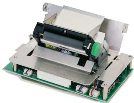
Gilbarco CRIND Printer with board Gilbarco # T20414-G1 PMP # 68315 used in T20490 G-4 Module (below)
