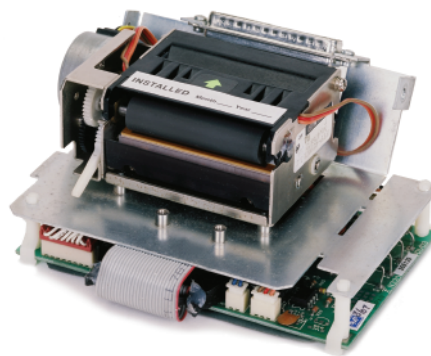
Gilbarco CRIND Printer with board Gilbarco # T18188-G4 PMP # 68308 used in T18188 G-5 Module (below)
