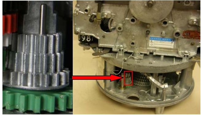
Figure 2b – Dollar Dive Shaft Gear Location
