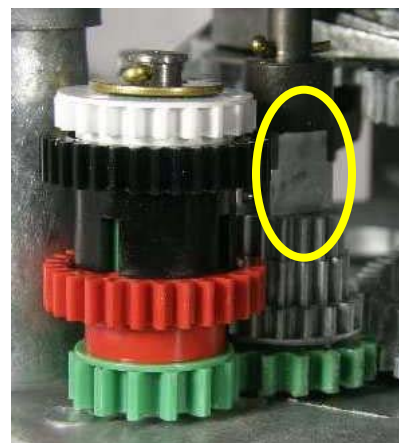
Vertical Pin Removed -Wrong! Figure 3b
